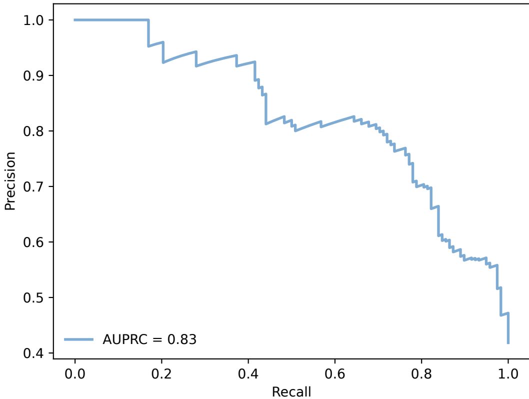
GBDT Precision-Recall Curve
